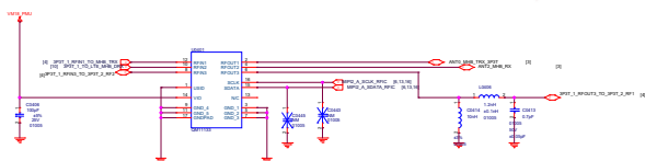
MHB 3P3T #1
