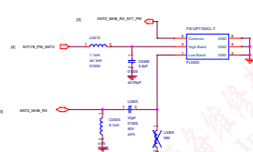
ANT2 DIP
