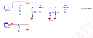
ANT5_B32+N78_1
