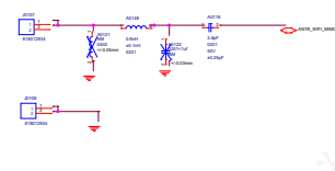
ANT8_WIFI CH1
